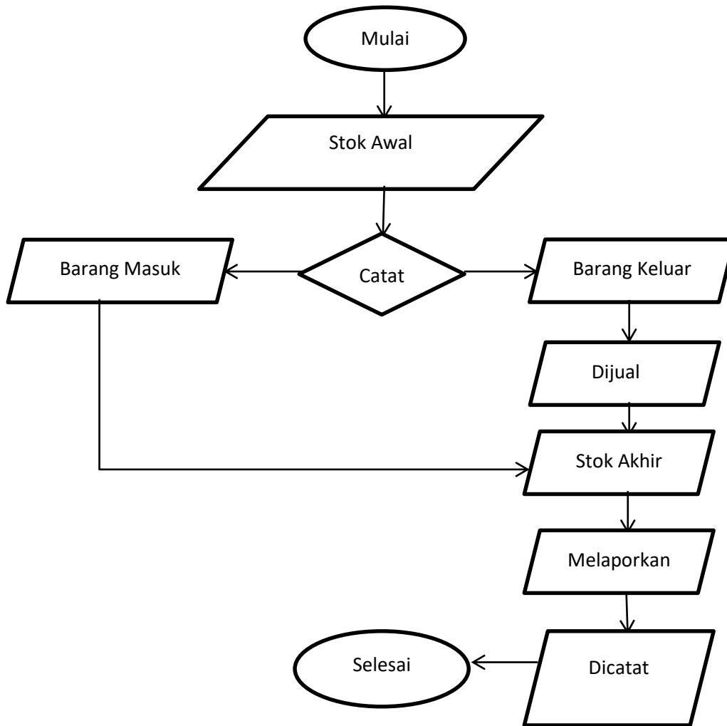
Gambar 1 Diagram Flowchart
